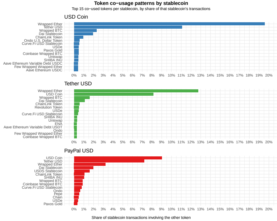
Figure 2. Co-usage patterns by stablecoin. For each stablecoin, the figure reports the most prominent co-used tokens and the share of that stablecoin's transactions in which each co-token appears within the same transaction. USDC and USDT share the same set of leading co-tokens, with the counterpart stablecoin in second place, indicating similar interaction patterns, while USDC exhibits stronger co-usage with Wrapped Ether, consistent with deeper integration into smart contract-based financial protocols. For PYUSD, stablecoins rank more prominently among the leading co-tokens, while overall co-usage is substantially lower.
