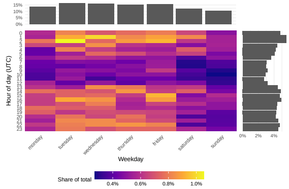
Figure 11. Heatmap of all Other transaction activity by stablecoin. Note repeated patterns during specific weekday/time-slots.
